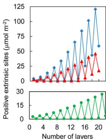
Figure 2. Positive bulk extrinsic sites (PDADMA + ) for (PDADMA/PSS) n PEMUs, n = 0-10 built in 0.5 M (◆) and 0.25 M NaCl (▲); and n = 0.5-11 for 0.1 M NaCl (●). The extrinsic sites are radiolabeled with ^{35}\text{SO}_4^{2-} ion by ion exchange in 1 \times 10^{-4} M \text{Na}_2^{35}\text{SO}_4 with a specific activity of 7.6 \text{ Ci mol}^{-1} . The amounts of extrinsic sites are presented as areal density, or \mu\text{mol m}^{-2} . Precision is \pm 3\% , and accuracy is \pm 5\% .
